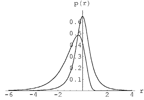
FIG. 1. Probability distributions for the estimation of squeezing on a vacuum input state. The asymmetric distribution comes from the suboptimal measurement of Ref. [7] in Eq. (16). The symmetric distribution corresponds to the optimal measurement of Eq. (12).
