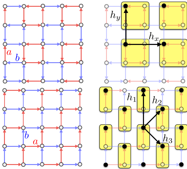
Fig. 3 From Ref. [27]. (Colors online). Two examples of reduction of a quantum walk on the Cayley graph of a virtually Abelian group G to that of a quantum walk on the Cayley graph of an Abelian subgroup H \subset G with finite index i_H . The graphs on the left of the figures are the Cayley graph of G (it is easy to see that both groups are non Abelian). The graphs on the right represents a choice of the Cayley graph of the subgroup H = \mathbb{Z}^2 , with the tiling corresponding to the induced representation (the elements of H are the black bullets). Top figures: G = \langle a, b \mid a^4, b^4, (ab)^2 \rangle . The index is i_H = 4 . The subgroup generators are h_x = a^{-1}b and h_y = ba^{-1} . The tiling is defined by the coset representatives e, a, a^2, a^3 . Bottom figures: G = \langle a, b \mid a^2b^{-2} \rangle . The index is i_H = 2 . The subgroup generators are h_1 = ba and h_2 = a^2 (or h_1 = ba and h_3 = ab^{-1} ), with the tiling the cosets representatives e, a
