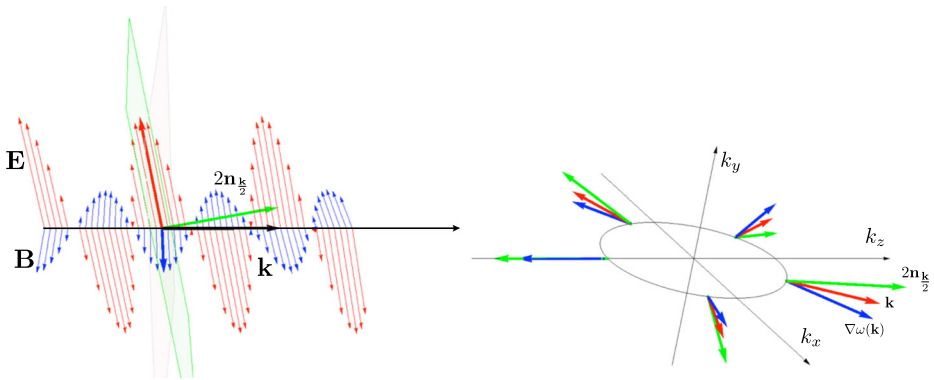
Fig. 5 From Ref. [14]. (Colors online). Left: In a rectilinear polarized electromagnetic wave, the polarization plane (in green) is slightly tilted with respect the plane orthogonal to \mathbf{k} (in gray). Right: vector 2\mathbf{n}_{\mathbf{k}}/2 (in green), which is orthogonal to the polarization plane; wavevector \mathbf{k} (in red) and group velocity (in blue) for the value |\mathbf{k}| = 0.8 and different directions. Notice that the three vectors are not parallel (the angles between them depend on \mathbf{k} )
