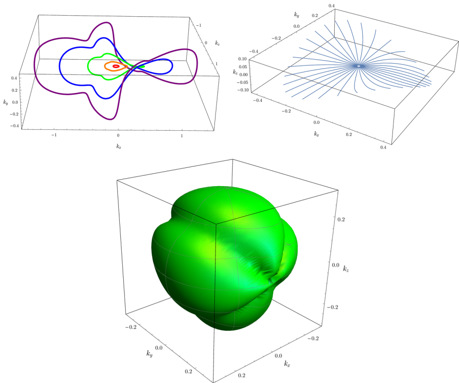
Fig. 6 From Ref. [15]. (Colors online). The distortion effects of the Lorentz group in the present quantum walk theory leading to the Weyl quantum field in the relativistic limit. Top left figure : the orbit of the wavevectors \mathbf{k} = (k_x, 0, 0) , with k_x \in \{.05, .2, .5, 1, 1.7\} under the rotation around the z axis. Top right figure : the orbit of wavevectors with |\mathbf{k}| = 0.01 for various directions in the (k_x, k_y) plane under the boosts with \beta parallel to \mathbf{k} and |\beta| \in [0, \tanh 4] . Bottom figure : the orbit of the wavevector \mathbf{k} = (0.3, 0, 0) under the full rotation group SO(3) .
