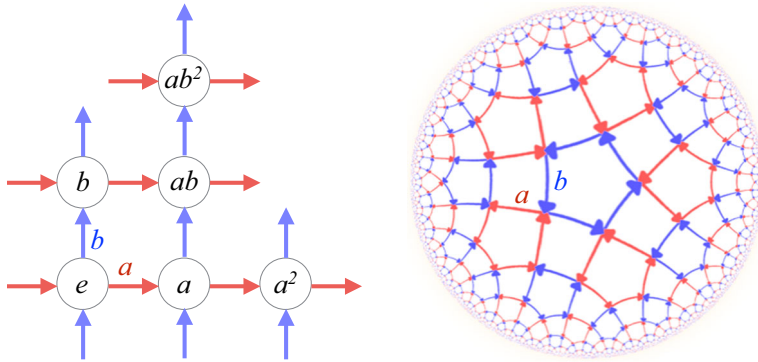
Fig. 2 From Ref. [26]. (Colors online). Given a group G and a set S_+ of generators, the Cayley graph \Gamma(G, S_+) is defined as the colored directed graph having set of nodes G , set of edges \{(g, gh); g \in G, h \in S_+\} , and a color assigned to each generator h \in S_+ . Left figure : the Cayley graph of the Abelian group \mathbb{Z}^2 with presentation \mathbb{Z}^2 = \langle a, b | aba^{-1}b^{-1} \rangle , where a and b are two commuting generators. Right figure : the Cayley graph of the non-Abelian group G = \langle a, b | a^5, b^5, (ab)^2 \rangle . The Abelian-group graph is embedded into the Euclidean space \mathbb{R}^2 , the non-Abelian G into the Hyperbolic space \mathbb{H}_2 with negative curvature
