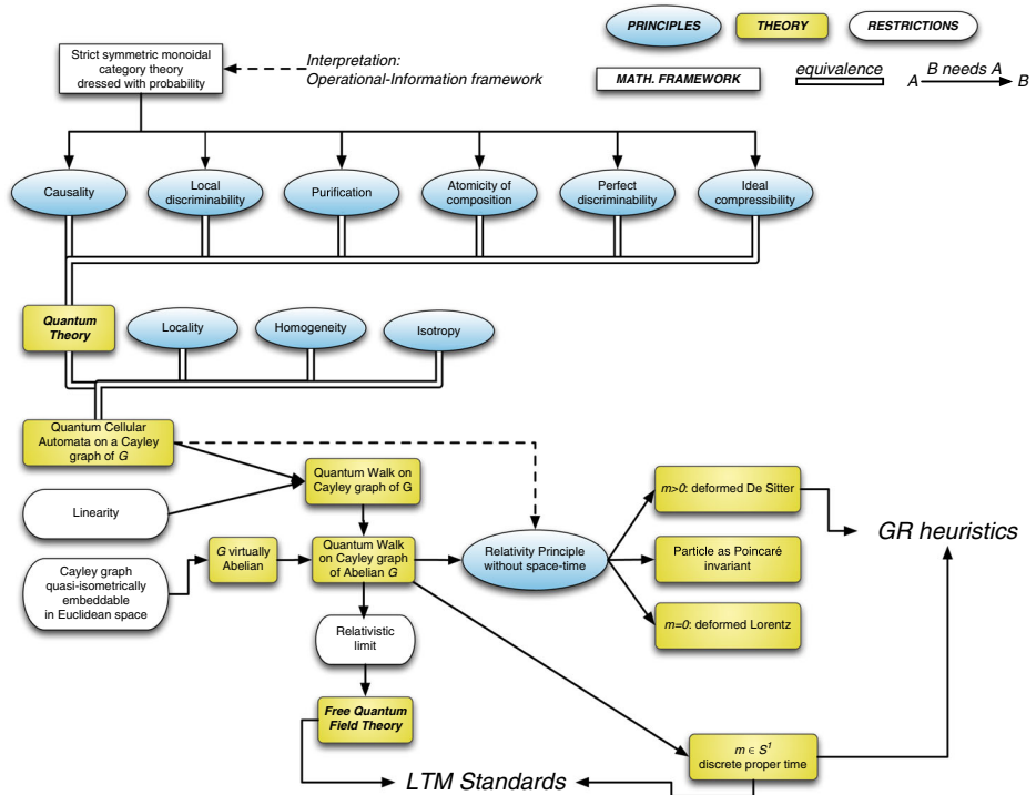
Fig. 7 Logical scheme of the derivation from principles of the present quantum-walk theory of fields, with the known free quantum field theory as its relativistic limit. The top six principles from which quantum theory of abstract system is derived are not discussed in the present paper, and can be found in Refs. [18, 25]
