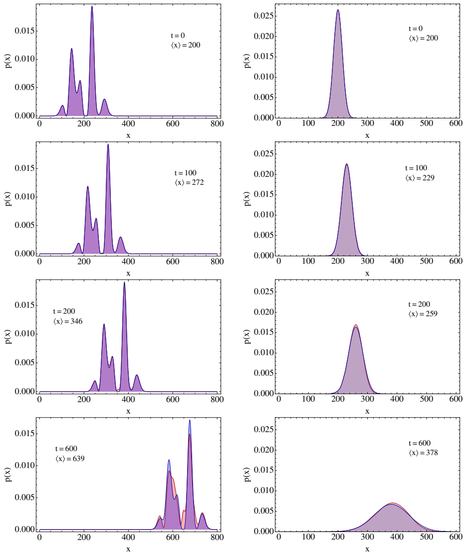
Fig. 4 From Ref. [11]. (Colors online). Test of the quality of the approximation of the Schrödinger (14) at for different time t of the Dirac quantum walk with mass m = 0.6 in one space dimension of Ref.[11]. Comparison of the probability distribution (in red) and the solution of the Schrödinger equation (in blue). Right figures : the state is a superposition of Hermite functions multiplied by the Gaussian peaked around momentum k_0 = 3\pi/10 , for drift and diffusion coefficients v = 0.73 and D = 0.31 , respectively. The mean value moves at the group velocity given by the drift coefficient v . The approximation remains accurate even for position spread \hat{\sigma} = 20 Planck lengths. Left figures : The same four times comparison for the quantum walk with m = 0.4 , and an initial Gaussian state peaked around the momentum k_0 = 0.1 . In this case the drift velocity and the diffusion coefficient are respectively v = 0.22 and D = 2.30
