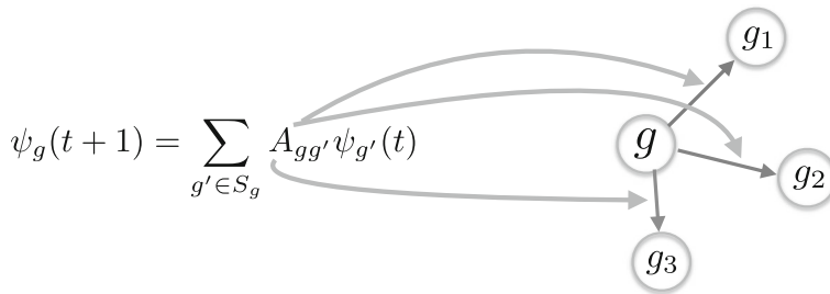
Fig. 1 The linear (3) endows the set G with a directed graph structure . We build a directed graph with an arrow from g to g' wherever the two are connected by a nonnull matrix A_{gg'} in (3)
